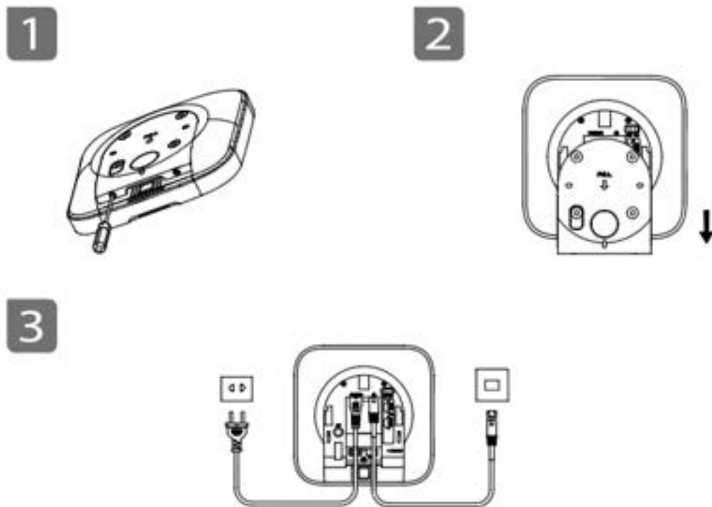
Figure 3-4 Power on
