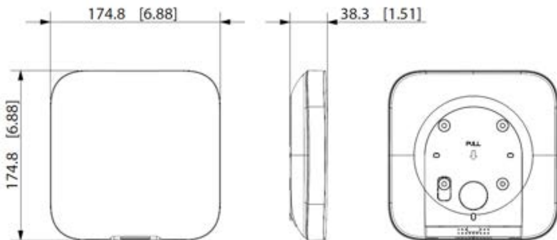
Figure 2-2 Dimensions (Unit: mm[inch])
